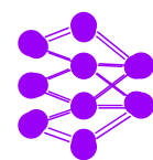
Data Mesh
