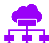
Data Hub
